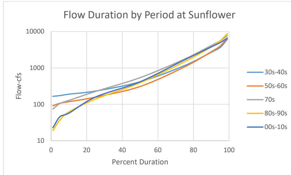
Figure 4-1. Flow Duration by Period in the Big Sunflower River at Sunflower, Mississippi
