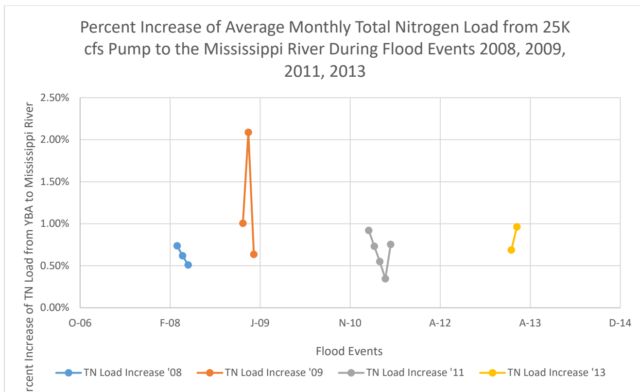
FIGURE 3-12. Theoretical Percent Increase of TN Load from the YBA to the Mississippi River during Previous Flood Events: 2008, 2009, 2011, and 2013.
