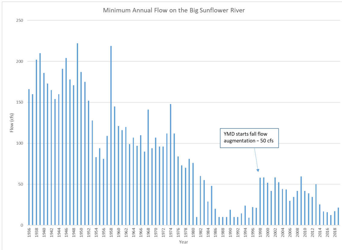
Figure 4-2. Annual Minimum Flow of the Big Sunflower River at Sunflower, Mississippi from 1936 to 2008.
