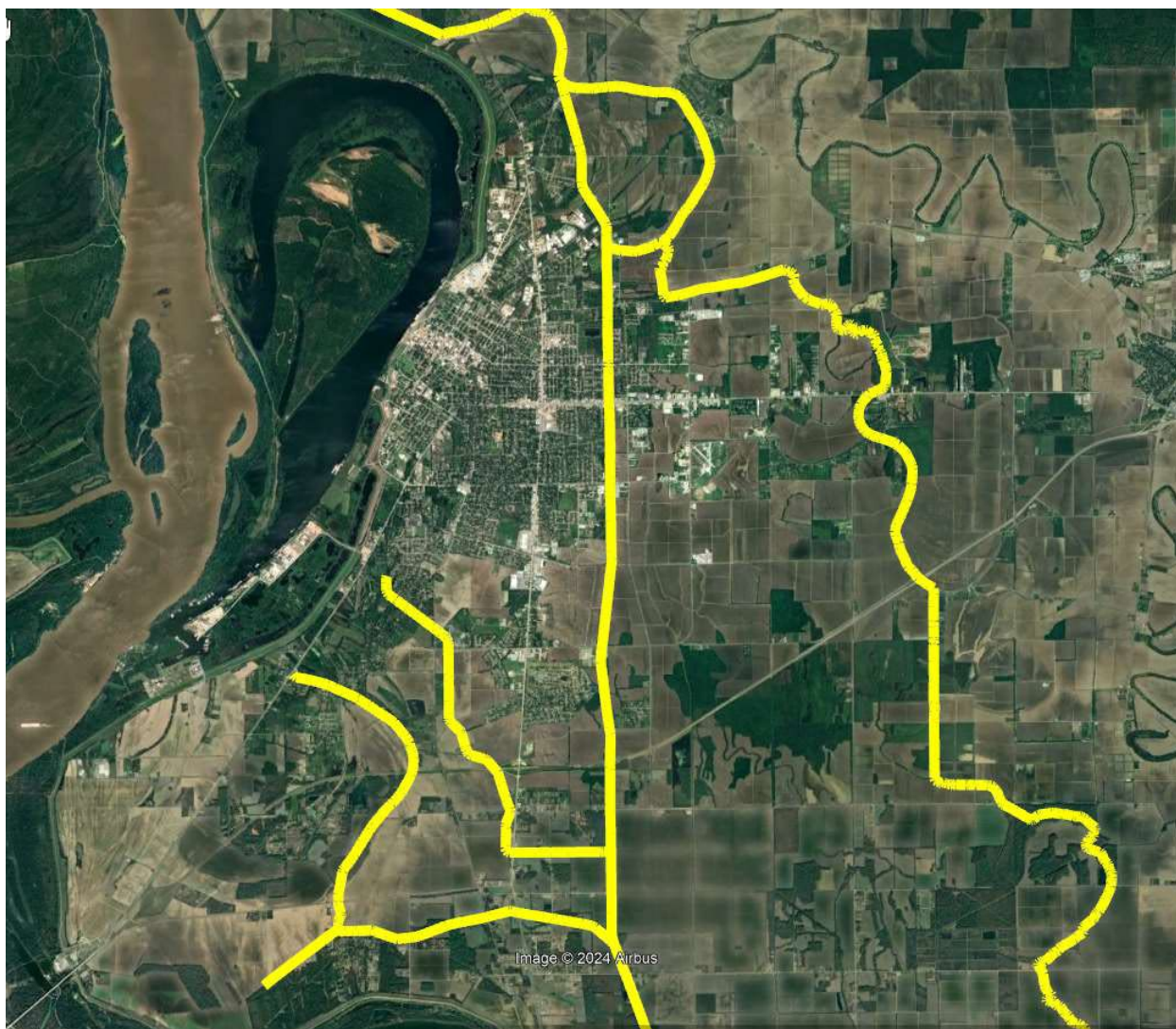
Figure 4-5. Map of the proposed 8 well sites for the Steele Bayou Basin along with the tributaries that will be supplemented.
