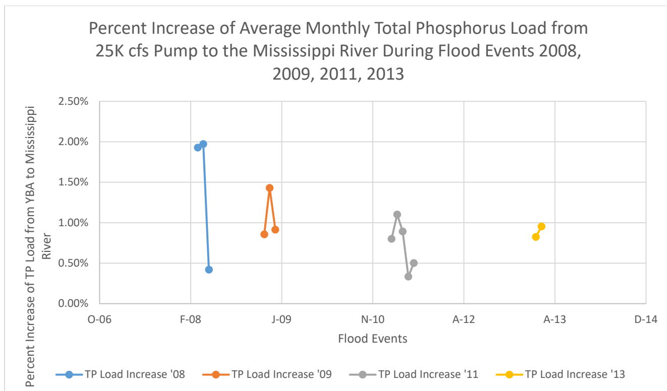
Figure 3-6. Theoretical Percent Increase of TP Load from the YBA to the Mississippi River during Previous Flood Events: 2008, 2009, 2011, 2013.
