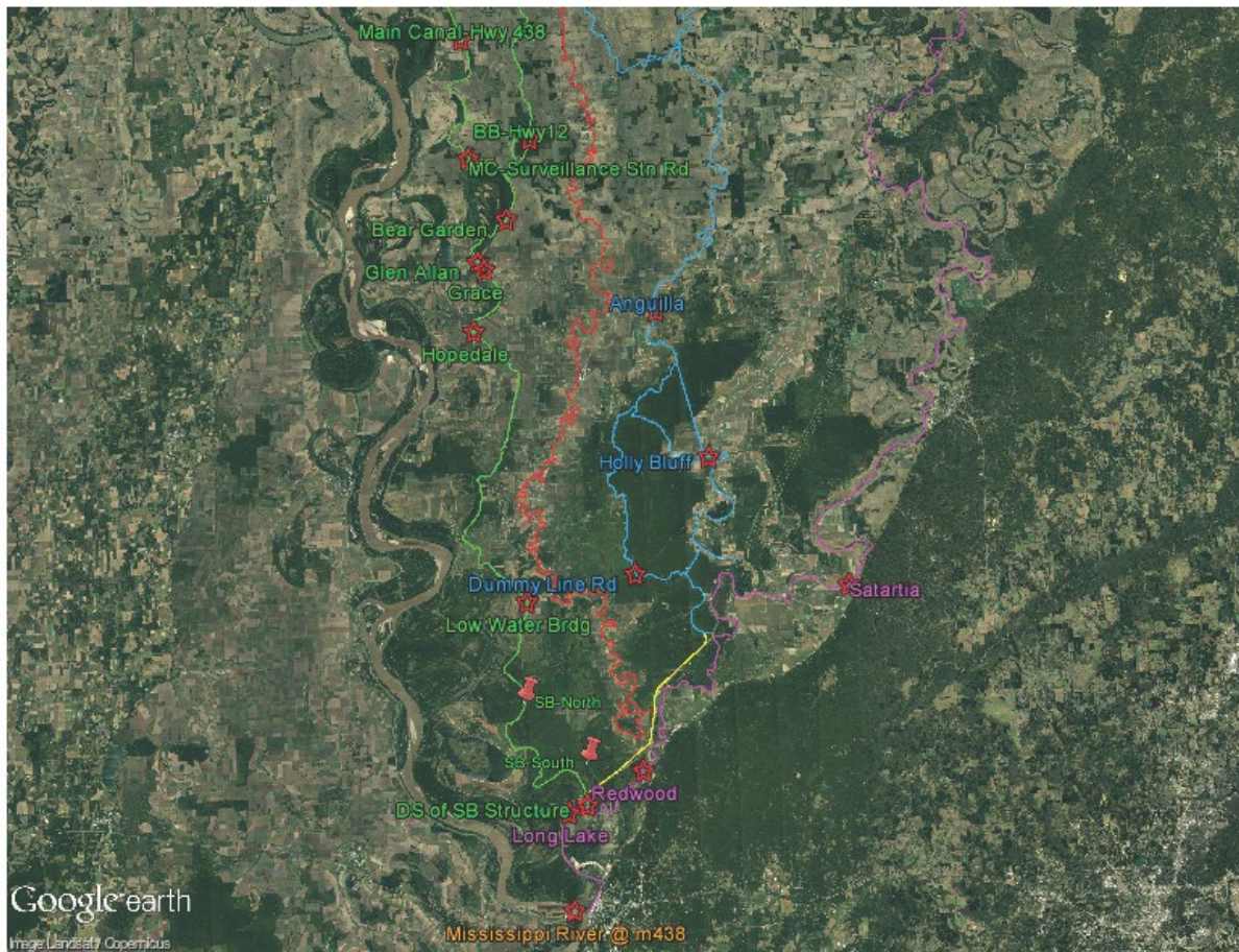
Figure 2-1. SBMP and NWIS stations utilized for deployment of water quality sondes and monthly grab samples.
