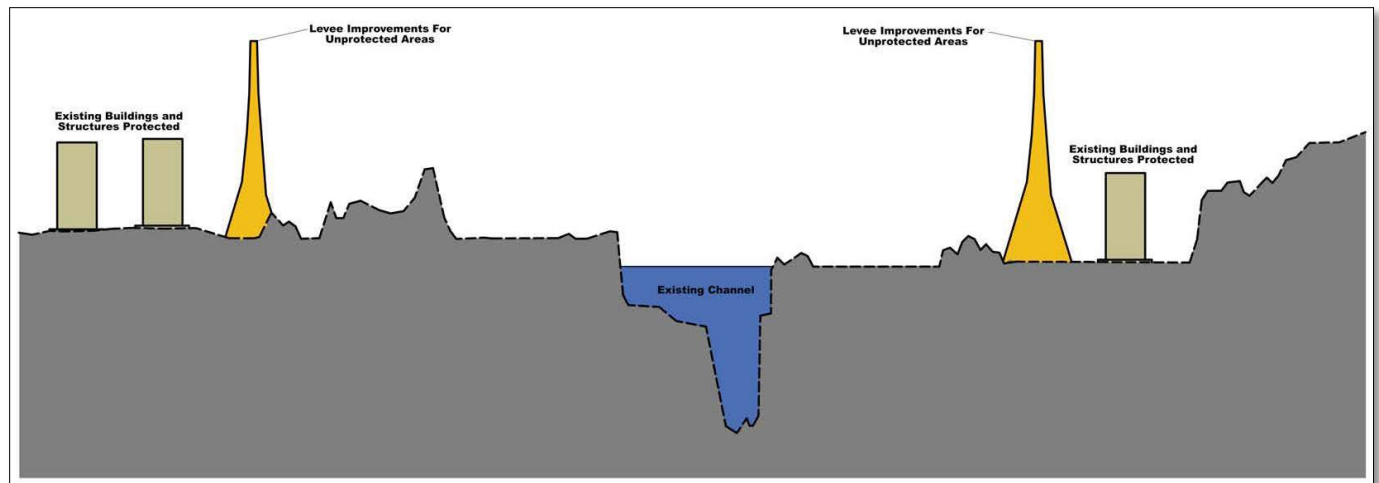
Figure 7-8. Levee Improvements for unprotected areas with existing buildings and structures.
