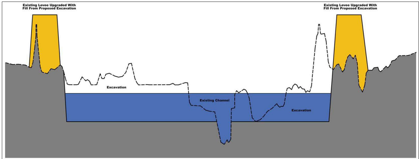
Figure 7-9. Channel Improvements with a relocated weir and improvements to existing levees.
