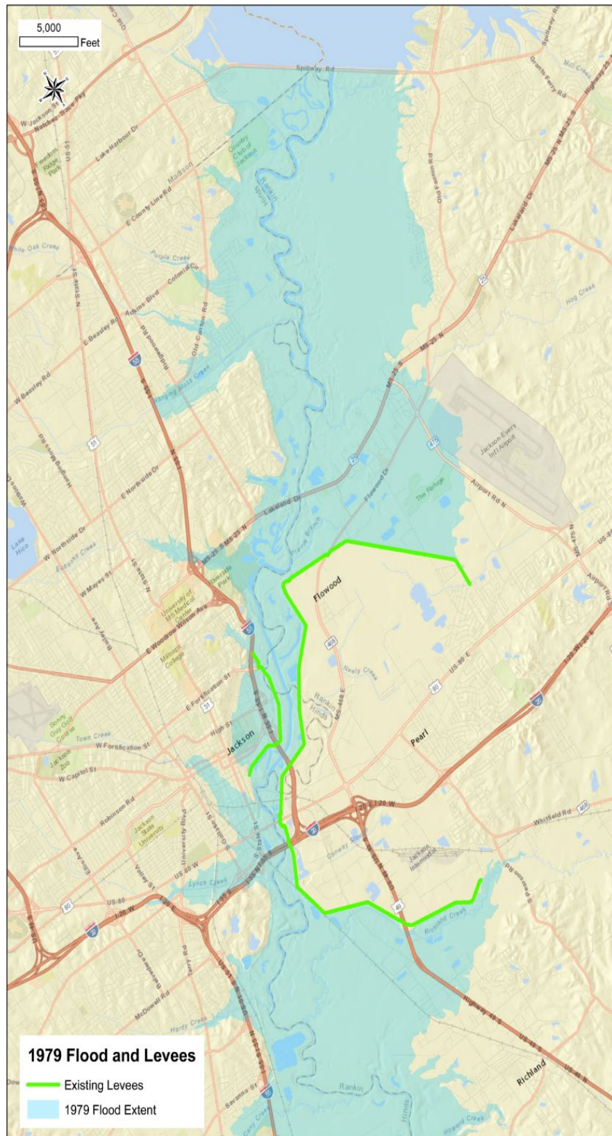
Figure 2-1. In 1979, the west section of the 13.5 mi levee protecting Jackson, MS was breached by floodwater. Shown are the locations of the levees and the extent of flooding during the 1979 event.
