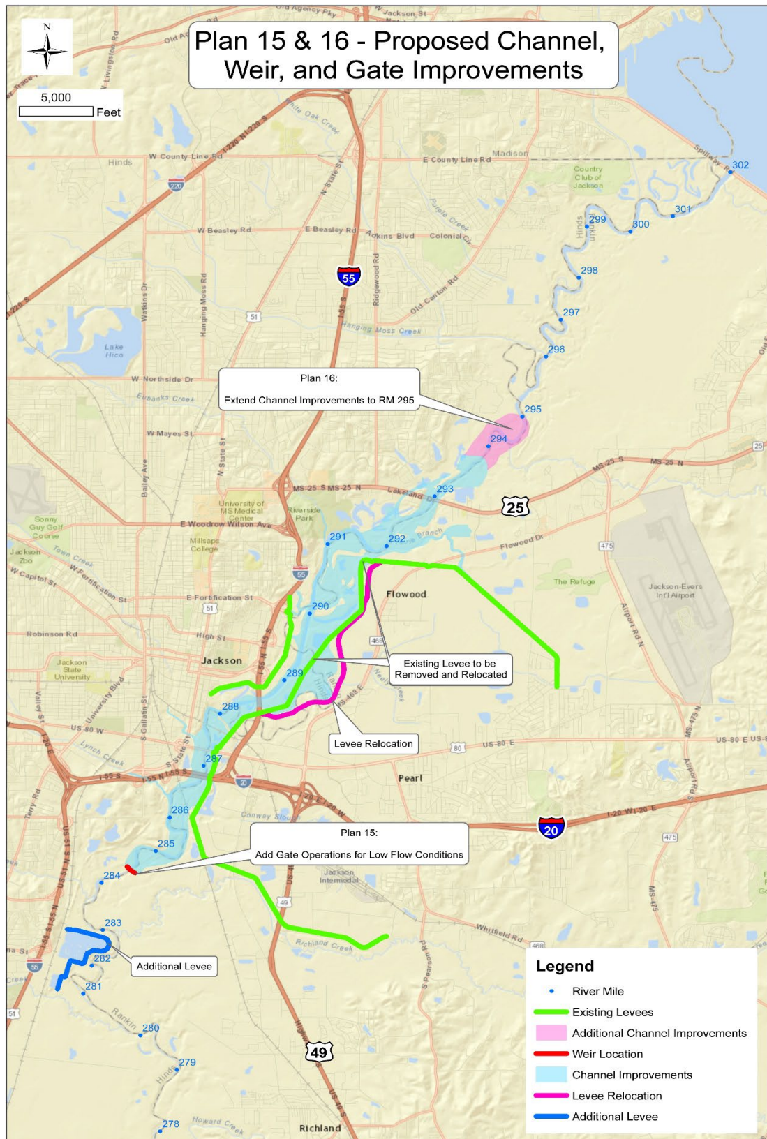
Figure 7-21. Similar to Plan 14, with the addition of gate operations at the weir (Plans 15 and 16) and the extension of channel improvements to RM 295 (Plan 16).
