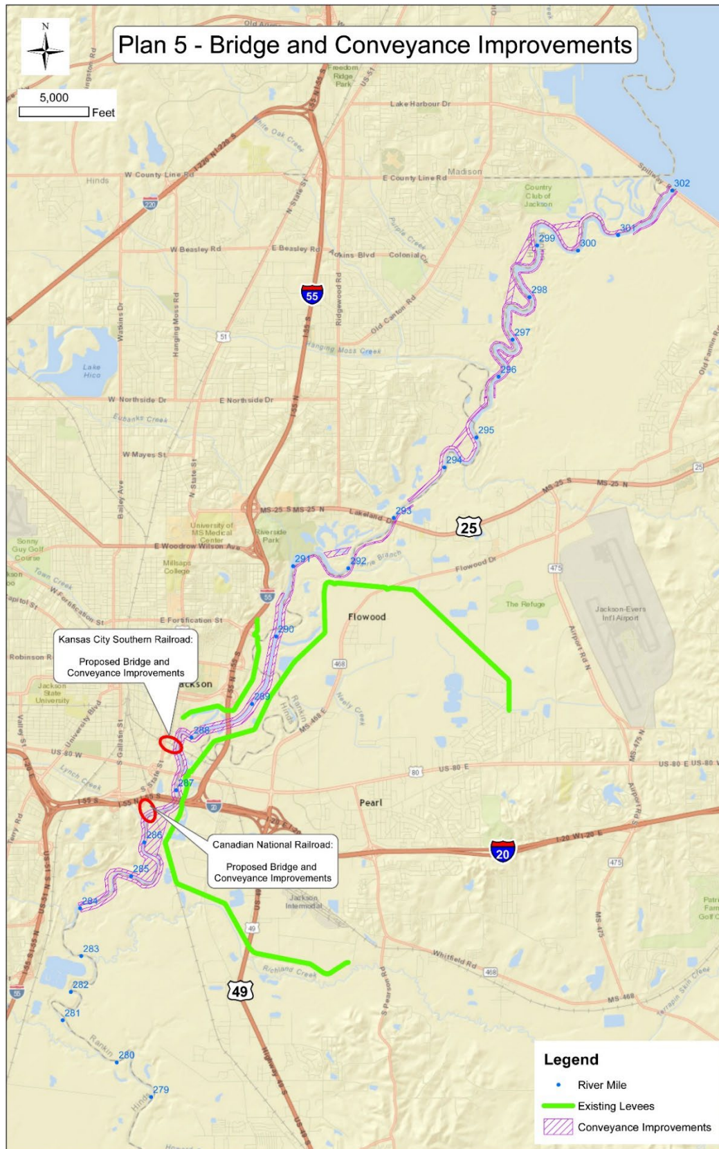
Figure 7-12. Conveyance and bridge improvements within the reach.
