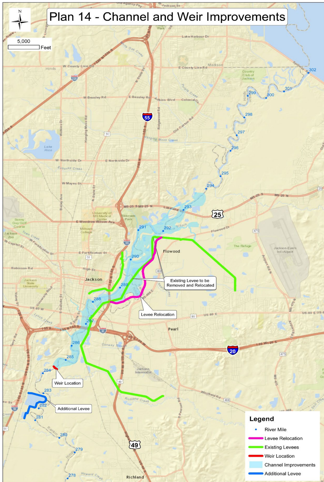
Figure 7-20. Channel improvements from RM 284 to RM 294, with weir relocation and additional levee around WWTP.
