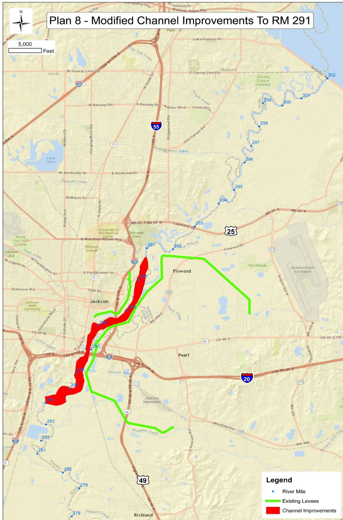
Figure 7-15. Channel improvements, with existing weir relocated to RM 284.
