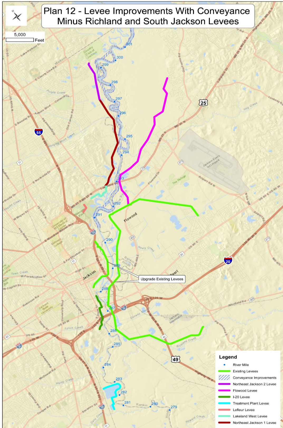
Figure 7-18. Similar to Plan 11, excluding Richland and South Jackson Levees.
