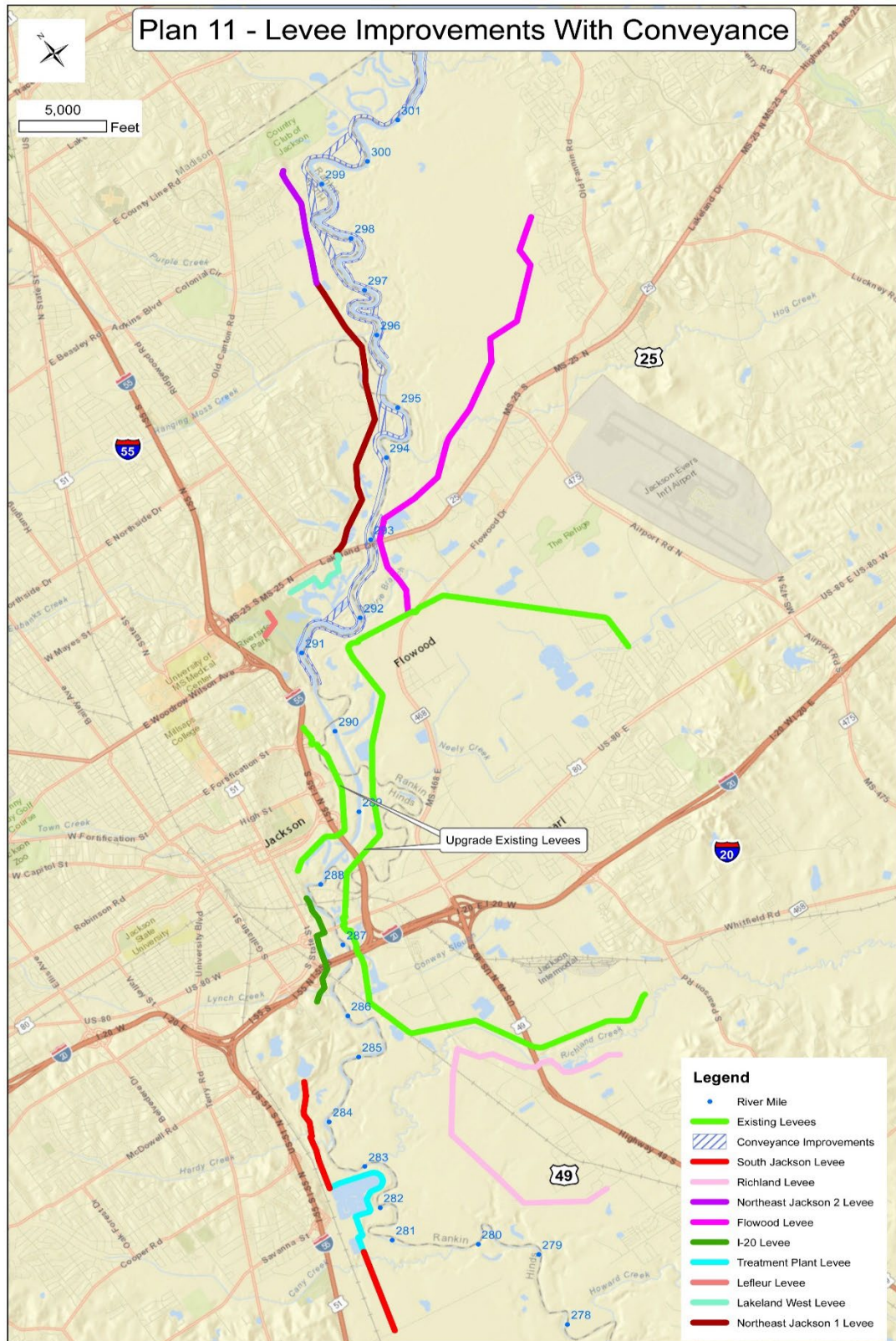
Figure 7-17. Additional levees and levee elevation improvements with conveyance improvements from RM 294 to RM 302.
